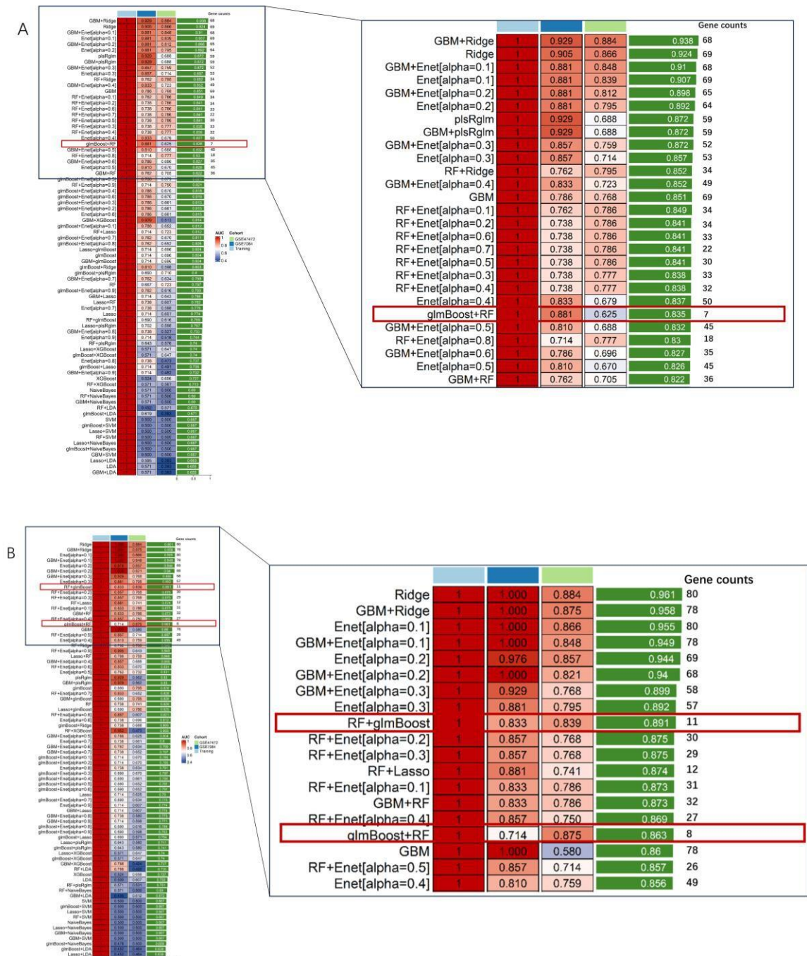
Fig S2 The AUC value of machine learning algorithms and the number of genes contained in the models. (A) The AUC values of machine learning algorithms and the number of genes included in the models when the top 100 differentially expressed genes were selected based on the threshold criteria of |\log_2FC| > 0.8 and FDR < 0.05 . (B) The AUC values of the machine learning algorithms and the number of genes included in the algorithms when the top 100 genes were selected based on the threshold of |\log_2FC| > 1.5 and FDR < 0.05 .
